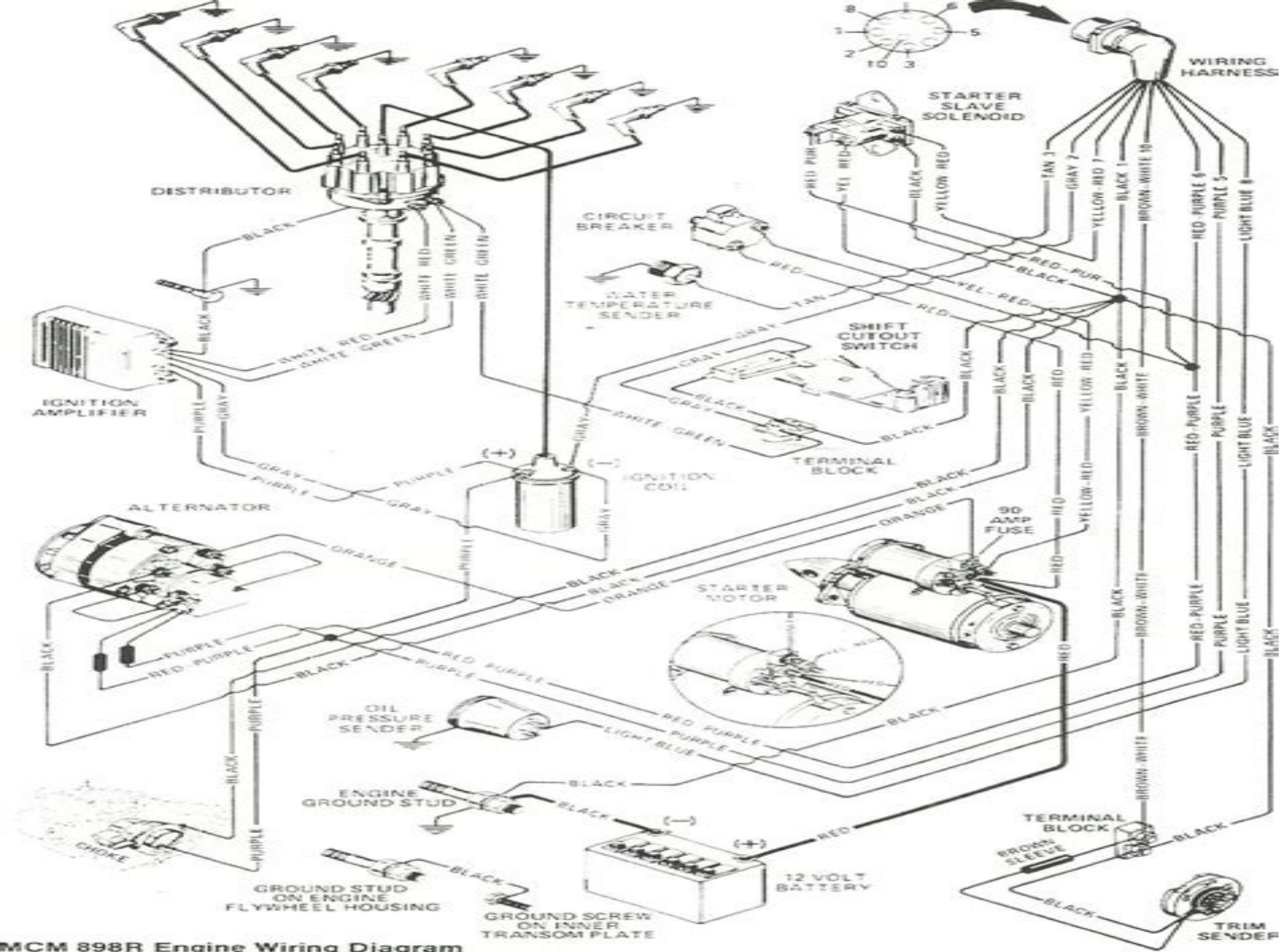
MCM 898R Engine Wiring Diagram Amp Fuse at Starter Motor (Orange Wire)
