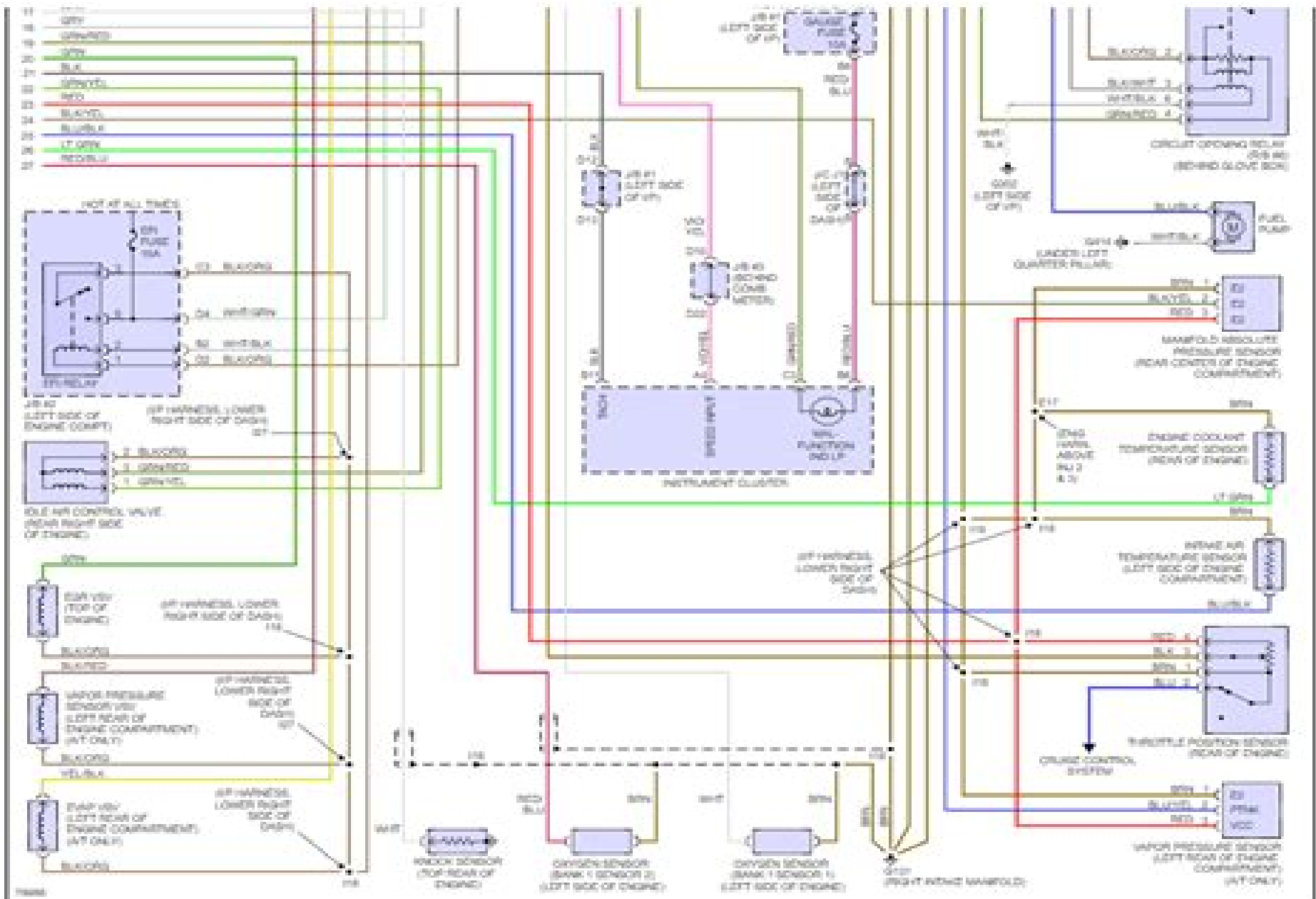
Fig 2: 2.2L, Engine Performance Circuits (2 of 2)
