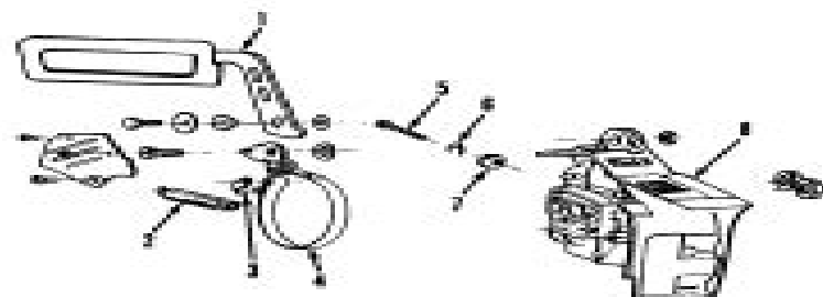
Fig. PN126—Exploded view of chain brake mechanism.
