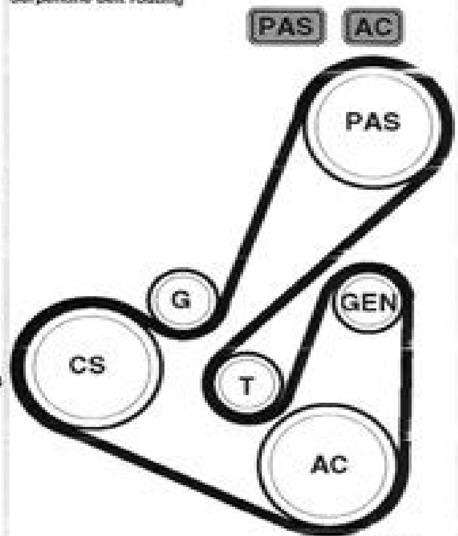
Serpentine belt routing
