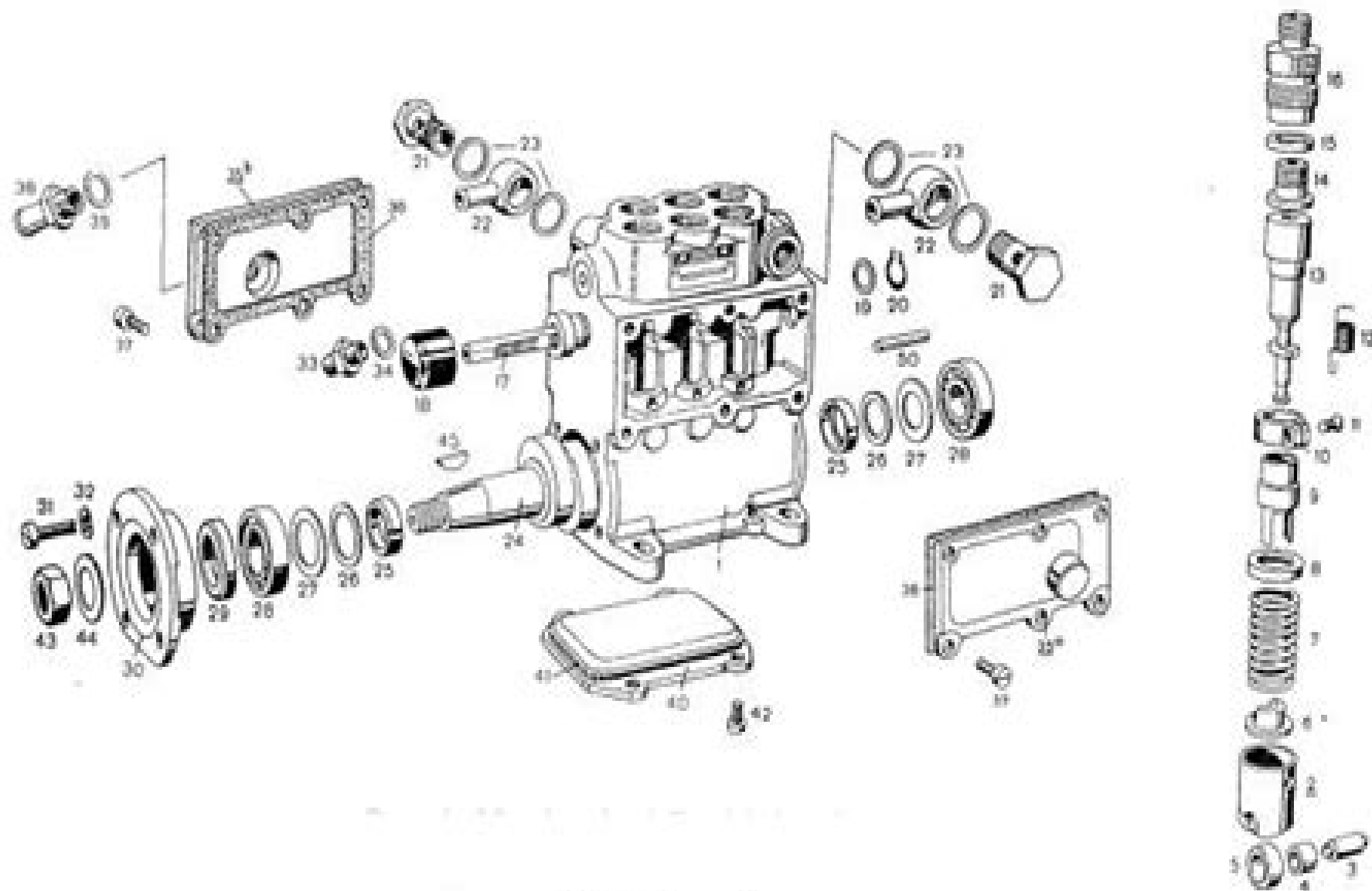
Pump
