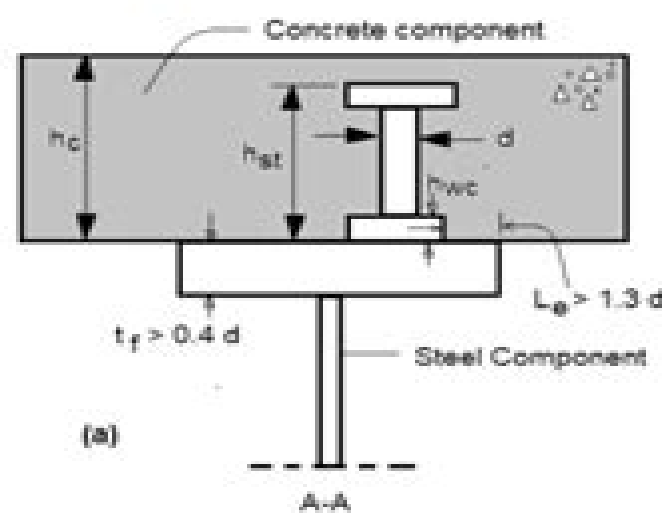
5. Proportioning of shear stud
