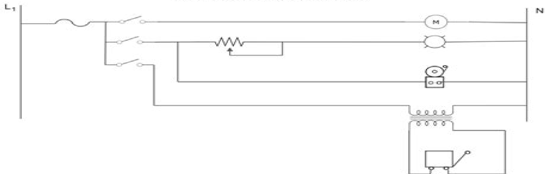
SCHEMATIC DIAGRAM
