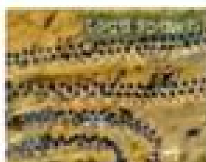
duckweed
