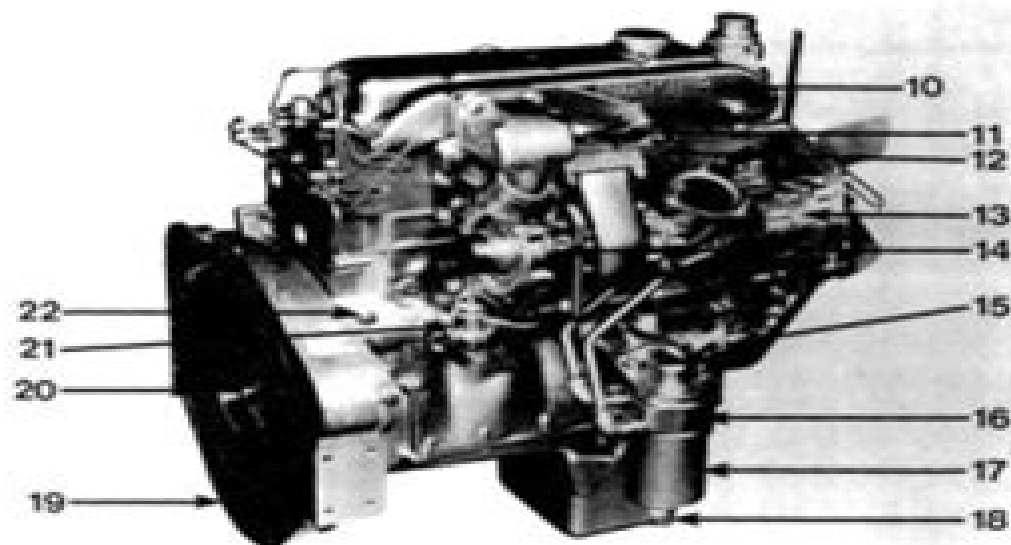
VIEW OF CAMSHAFT SIDE OF T4.236 ENGINE
