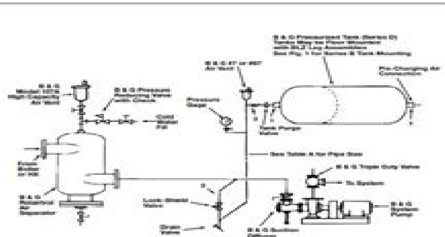
Figure 2 Horizontal Tank Installation with Rolairtrol Air Separator
