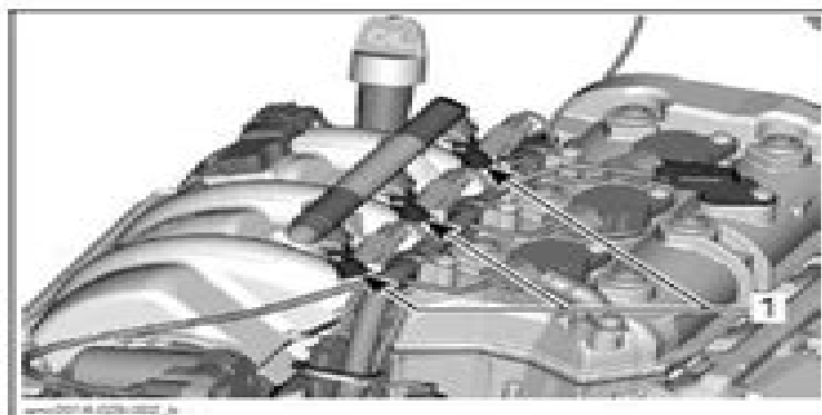
1. Fuel injectors
