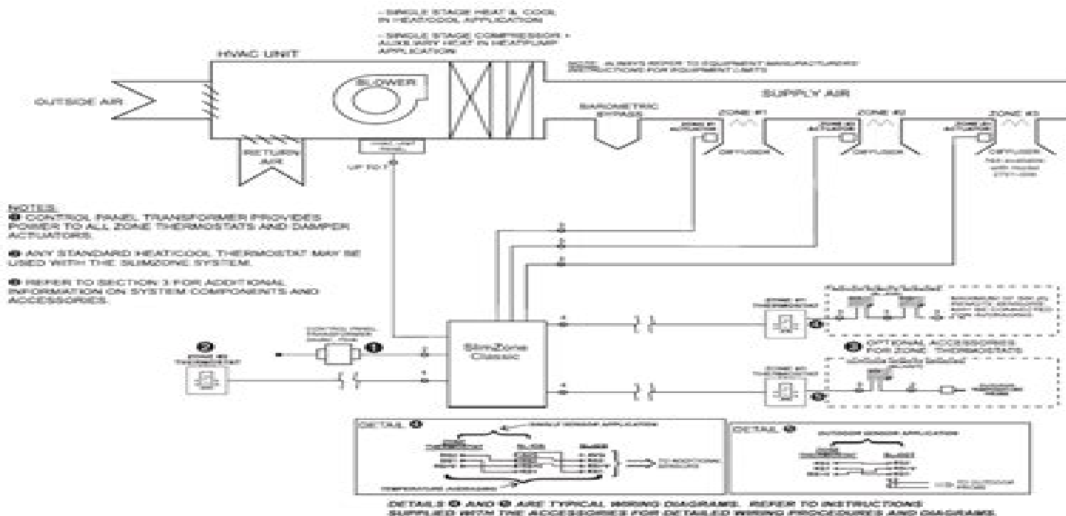
Figure 3.1: SlimZone Classic System Diagram
