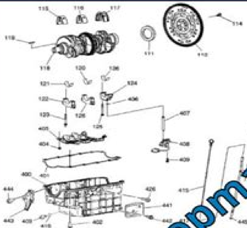
Fig. 4: View Of Crankshaft and Connecting Rod Assembly Courtesy of GENERAL MOTORS CORP.
