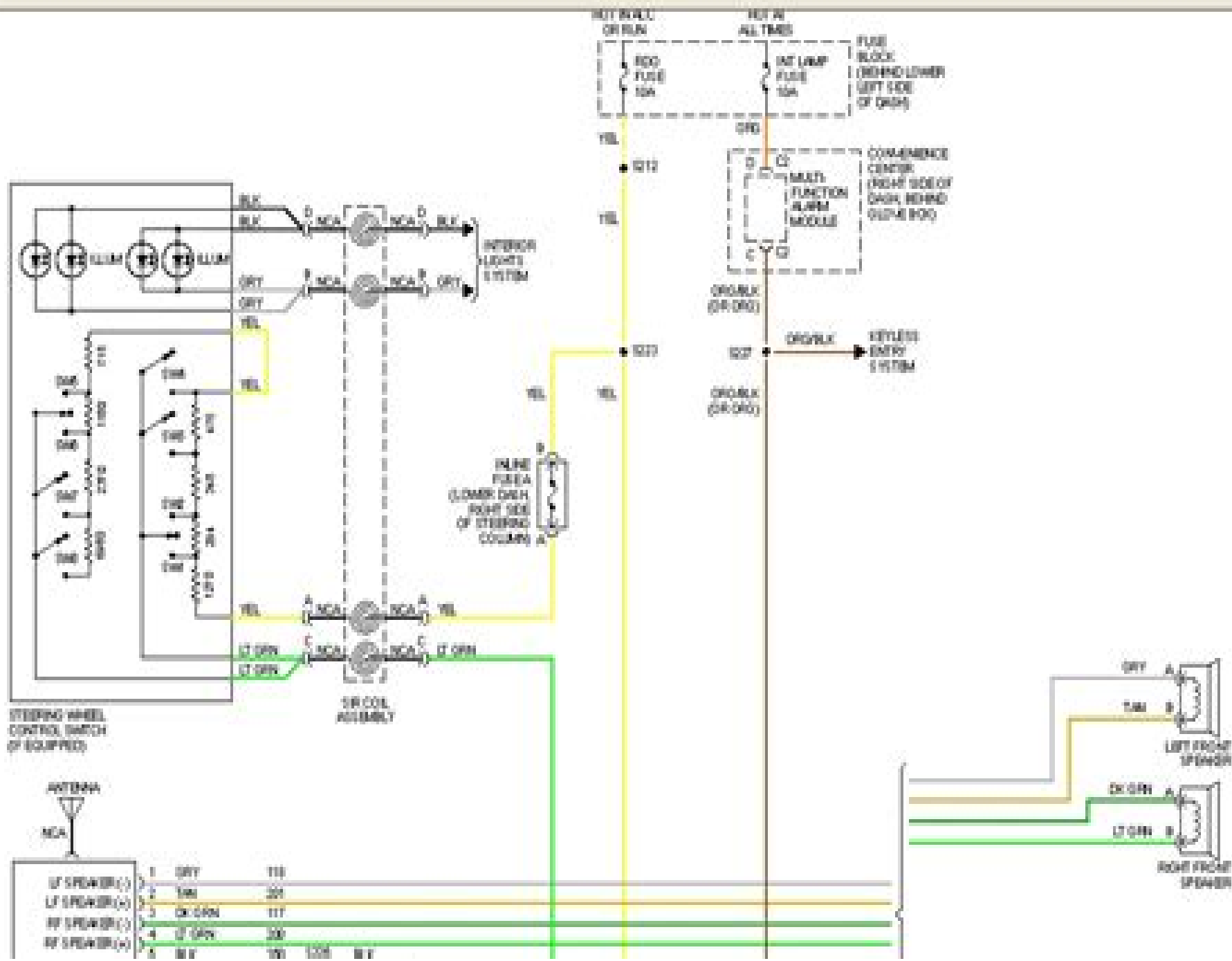
Fig. 34 Radio Circuitry
