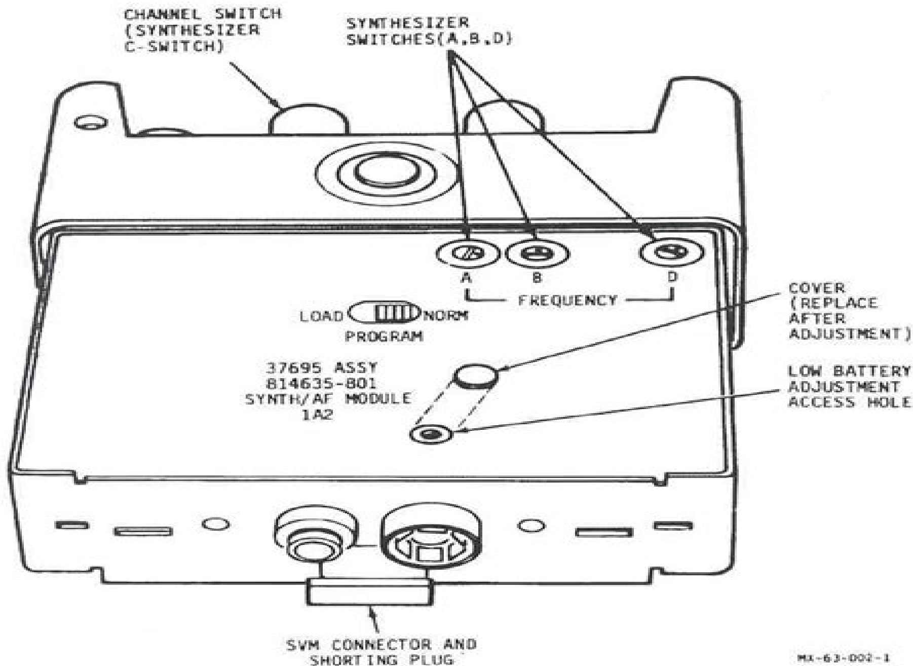
Figure 2-3. Radio Set Component Locations, Rear View
