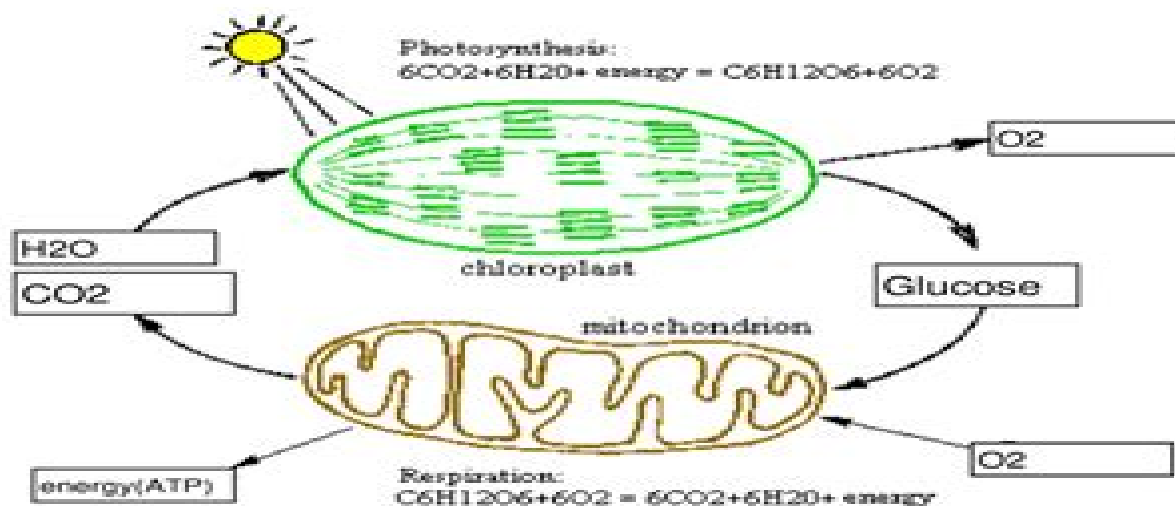
Figure 16- With the photosynthesis, the solar energy is converted by the chloroplasts as sugar molecules. With the glycolysis and the respiration, made by mitochondria, the energy is liberated and supplied to the cell for its biochemical processes.
