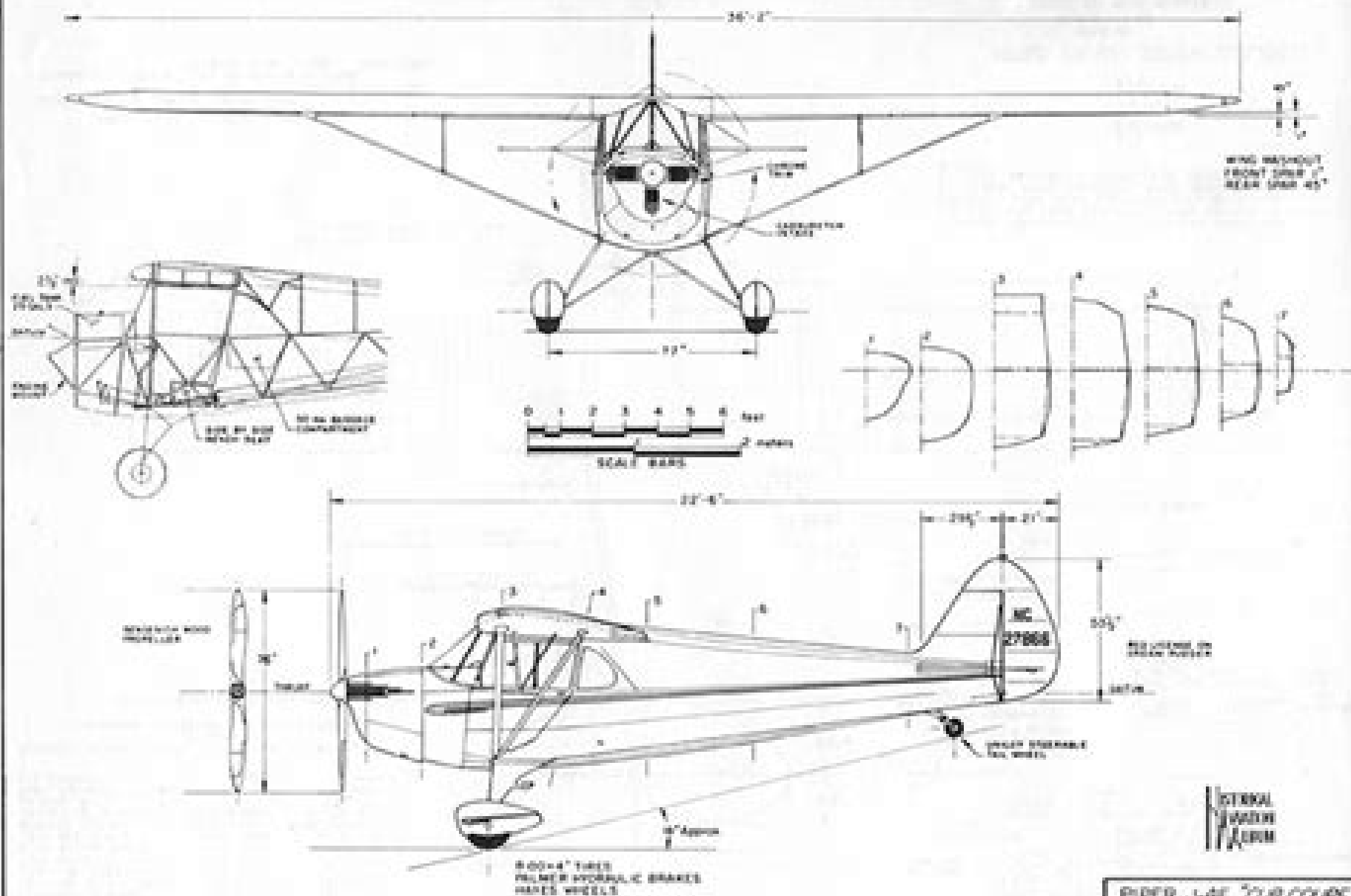
PIPER J-4E "CUB COUPE" 1941 MODEL SCALE: ORIGINAL - 1/24 REPROD. - 1/48 DRAWN BY PAUL R. WELT © HISTORICAL AVIATION MUSEUM 1988 P.O. BOX 23 TEMPLE CITY, CALIF. 91780
