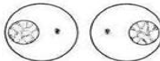
Daughter cells
