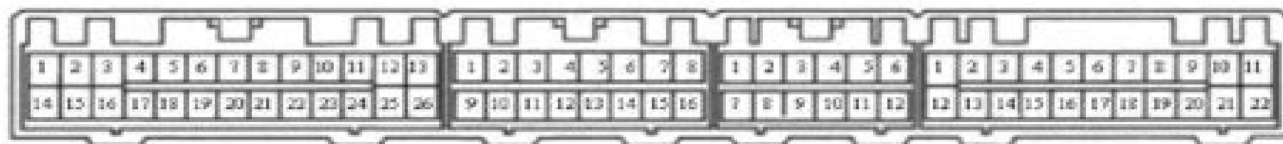
Connector 1 - C-33
