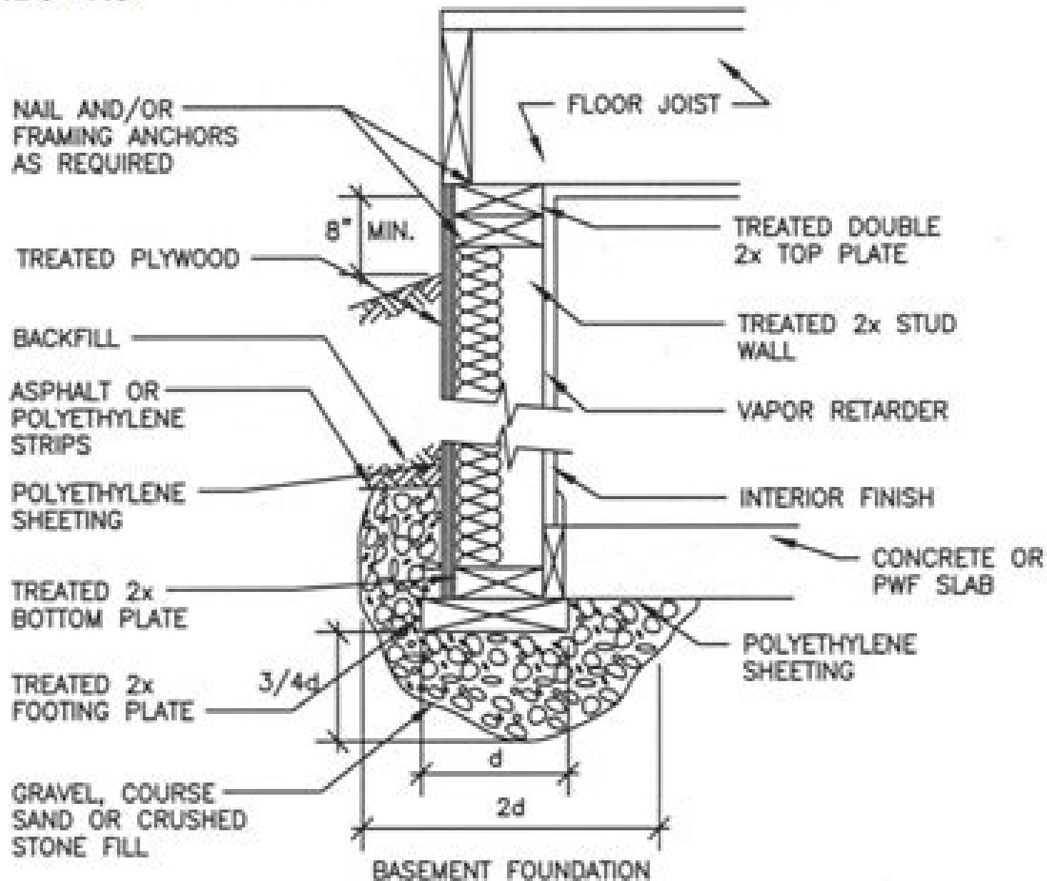
Figure 4.9 Preservative-Treated Wood Foundation Walls
