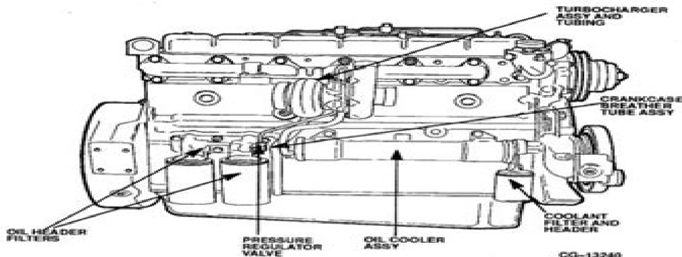
Figure 1.1. Component Removal Prior to Mounting the Engine on the Stand
